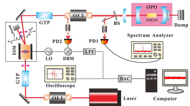
Fig. 2. Experimental setup for measuring the noise power spectrum of phase-modulated light and the ZBD of the PDH error signal. EOM, electro-optic modulator; GTP, Glan-Thompson prism; OI, optical isolator; BS, beam splitter; OPO, optical parametric oscillator; PPKTP, periodically poled \text{KTiOPO}_4 ; LO, local oscillator; DBM, doubly balanced mixer; PD, photodetector; LPF, low pass filter; DAC, data acquisition card.
